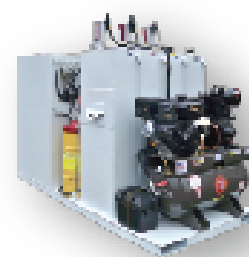
TPL 236-ERC-AC Three product + antifreeze + grease + 14hp compressor
