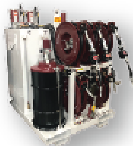
TPL 236-994 Three product + grease
